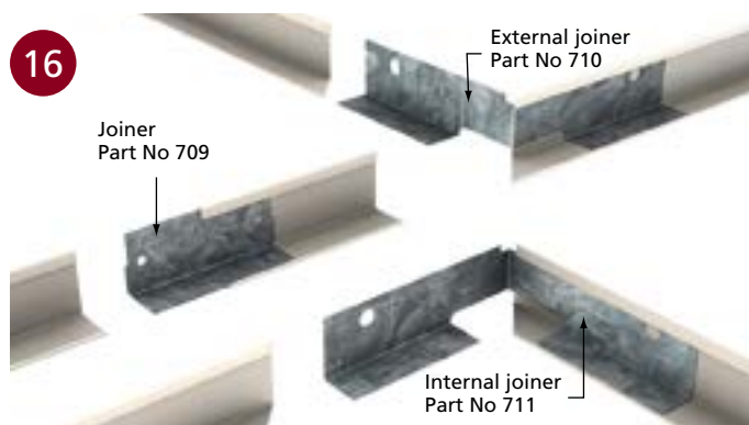
■ BULKHEAD JOINER DETAILS
