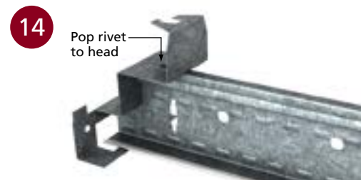
■ SUPPORT CLIPS
